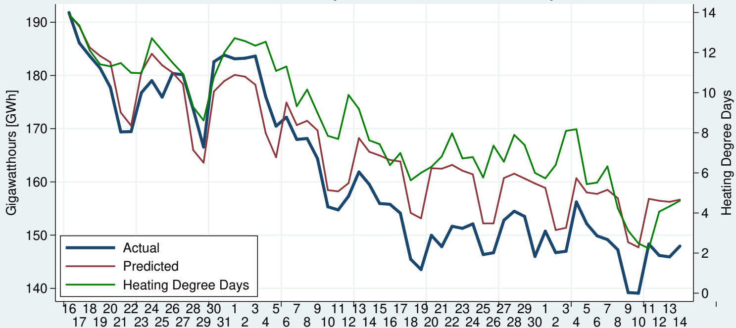
Actual and Predicted BC Hydro Load, March 16 – May 14, 2020
